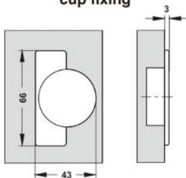
Drilling dimensions for cup fixing
