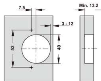
Drilling dimensions for cup fixing screw fixing
