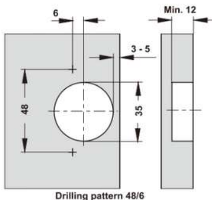
Drilling dimensions for cup fixing screw fixing
