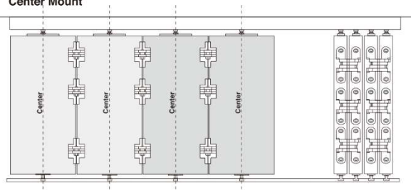
Center Mount
