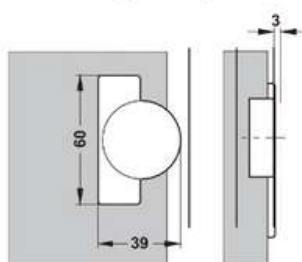
Drilling dimensions for cup fixing
