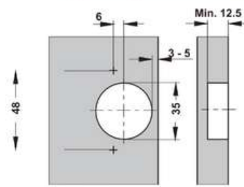
Drilling pattern 48/6
