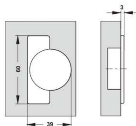
Drilling dimensions for cup fixing
