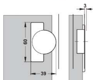
Drilling dimensions for cup fixing
