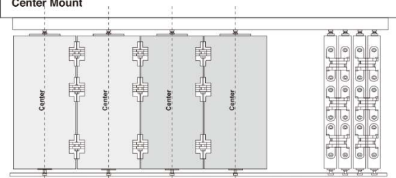
Center Mount
